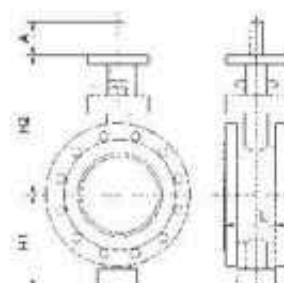
Double Flanged Type
