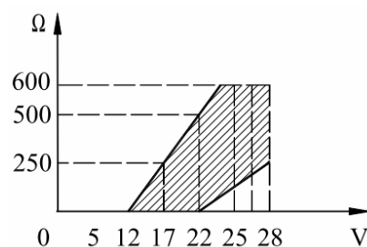
Load diagram
